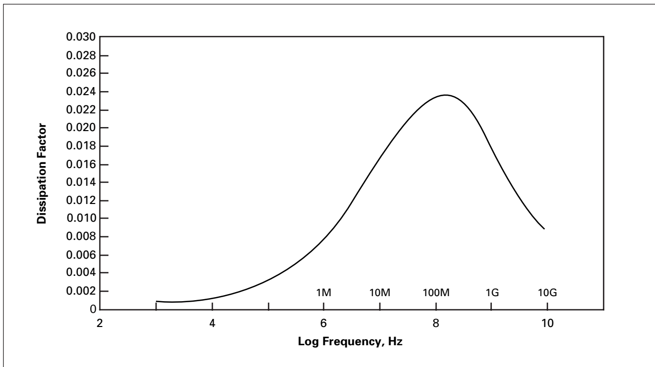
Figure 14. Tefzel 200 Dissipation Factor—Room Temperature
